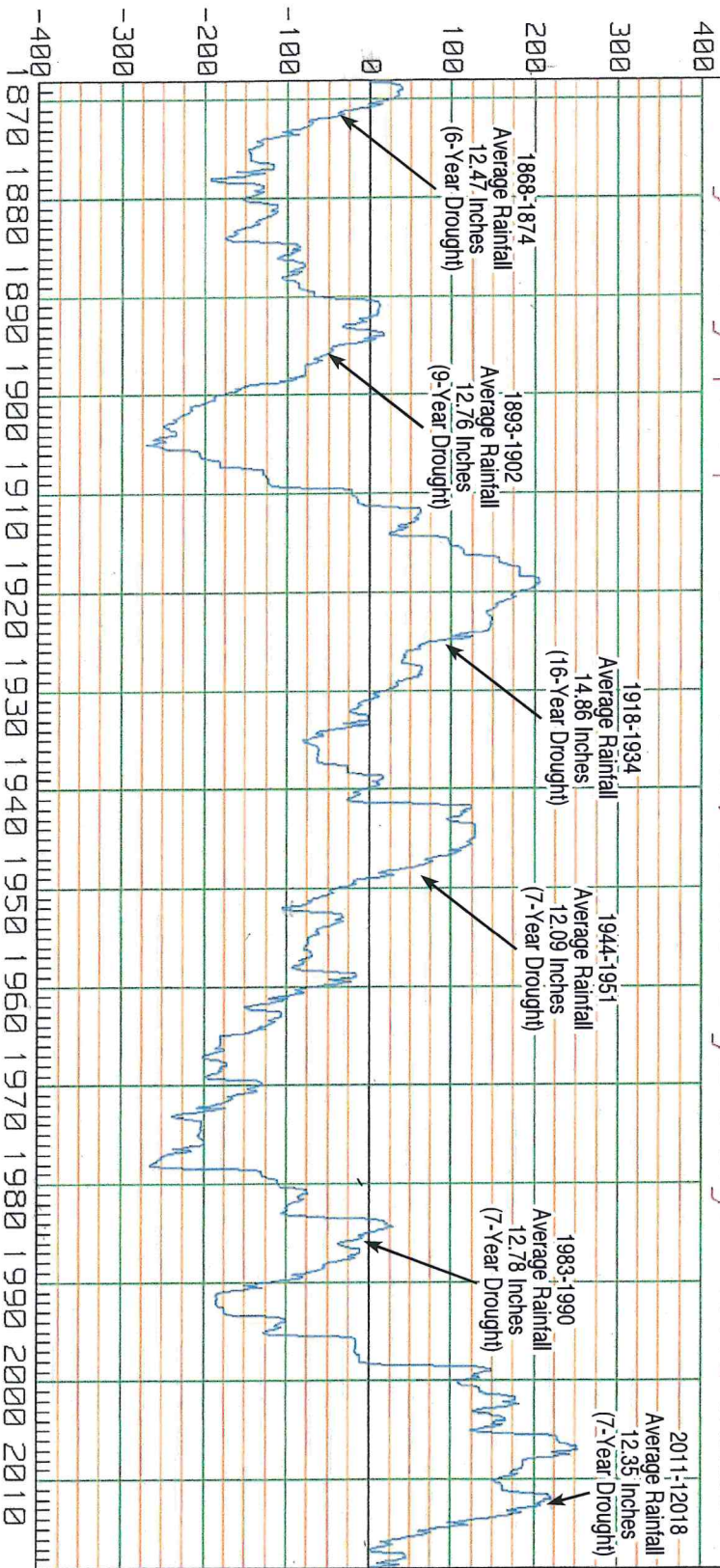
DEVIATION FROM MEAN IN %: TIME SCALE = SEPTEMBER-AUGUST WATER YEARS SHOWING PRIMARY DROUGHT CYCLES
