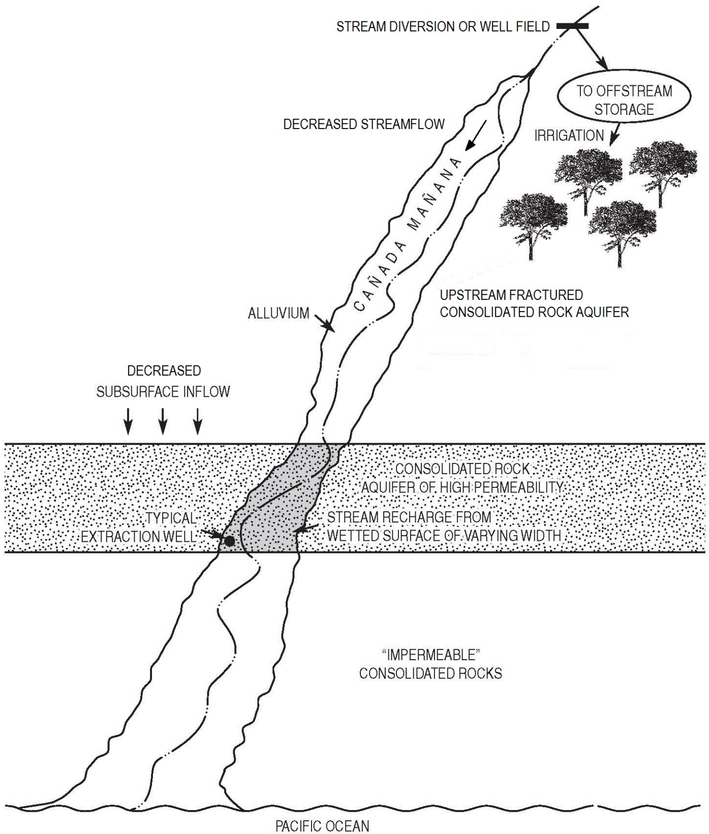
DIAGRAM SHOWING RELATIONSHIP OF UPSTREAM DIVERSION OR WELL FIELD TO DOWNSTREAM AQUIFER
